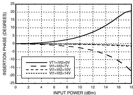
Rejection Band, Insertion Phase vs. Pin
