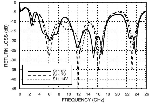
Broadband Return Loss ( S11 ) vs. Vt
